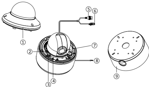
Figure 1-3 Overview of Type II Dome Camera
