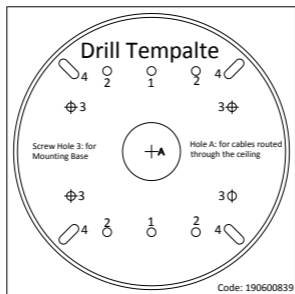
Figure 2-8 Drill Template
