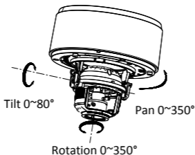
Figure 2-4 3-axis Adjustment
